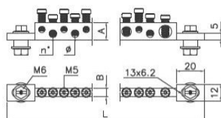
KL11-13-6-20 - KL11-13-6-50
