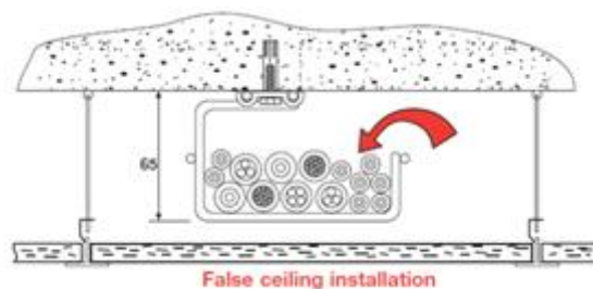
False ceiling installation
