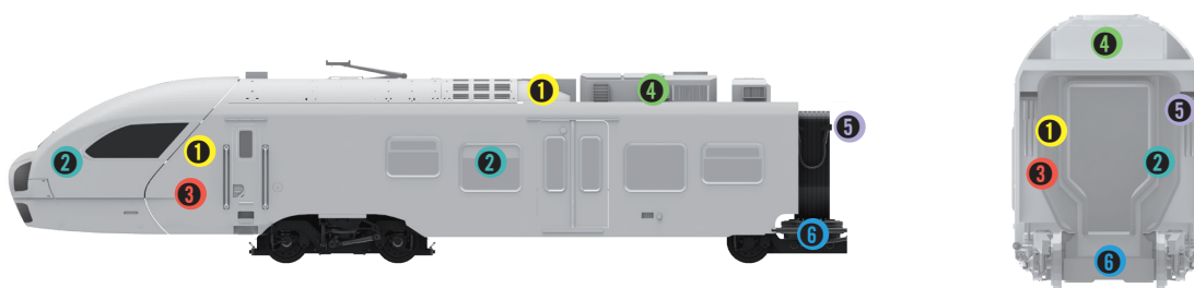
Figure A*: Typical connector locations on board rolling stock
