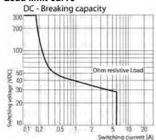
Load limit curve
